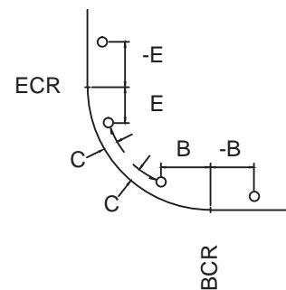
POLE PLACEMENT
